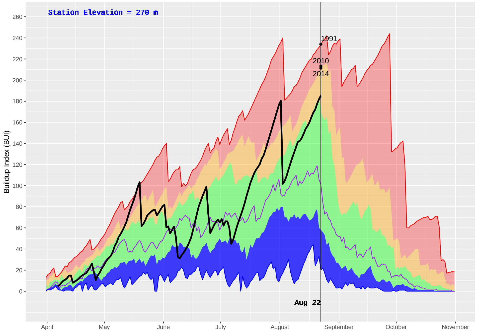
TALCHAKO (233) : Historical (1990–2016) and Current (2018) Daily Buildup Index (BUI)
